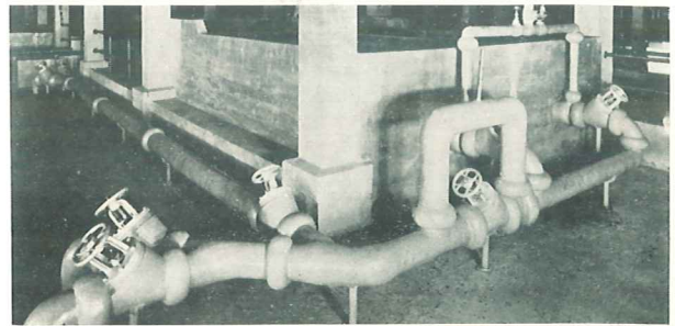
Above: Lead pipe line for handling a salt solution. Pipes are insulated to facilitate temperature control. Below: Discharge pipe on the outside of a circular concrete settling tank.
