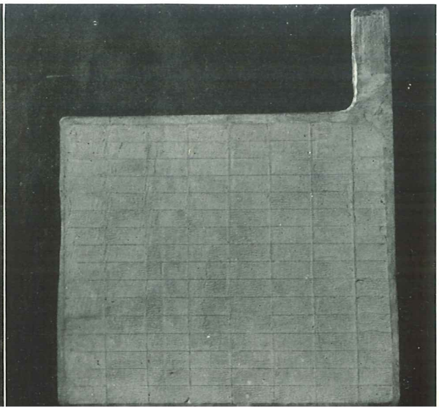
Above: Storage battery room in a large broadcasting studio. Note the lead grid inside the battery in the foreground. Below: Standard type of grid used in the automobile storage battery. The grid at the right is shown after pasting with lead oxide.
