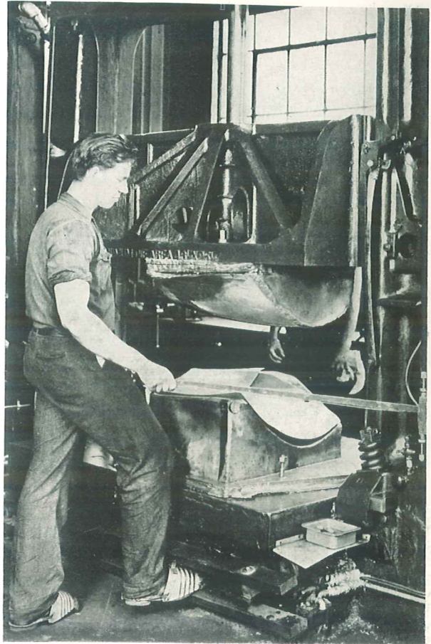
Right and left hand upper front door sill stampings, made of .037" deep-drawing body steel. 18,000 pairs were produced from die sets of Kirksite A. Two-foot Kirksite A shrinkage rule indicates relative size of stampings.
