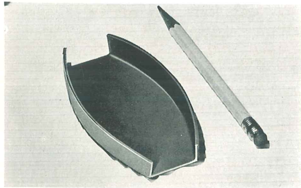
Using .062" steel, 1800 of these parts were blanked on one rolled Kirksite A die and formed on punch and die of cast Kirksite A. (Pencil indicates relative size.)
