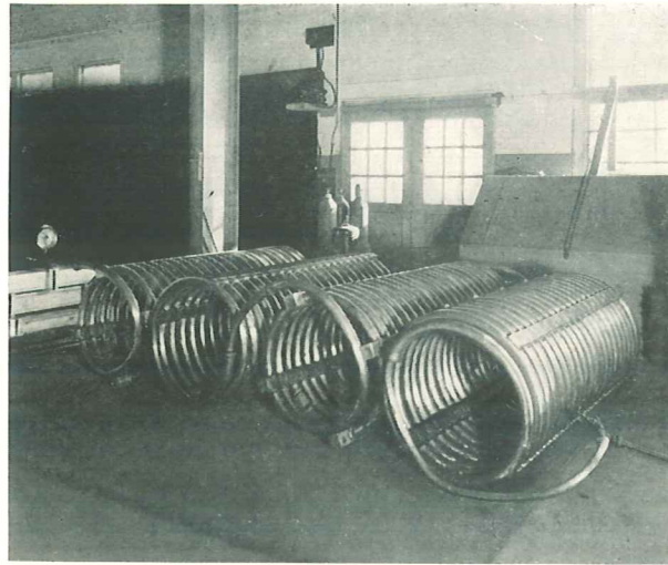
Special helical lead coils coupled for testing.
