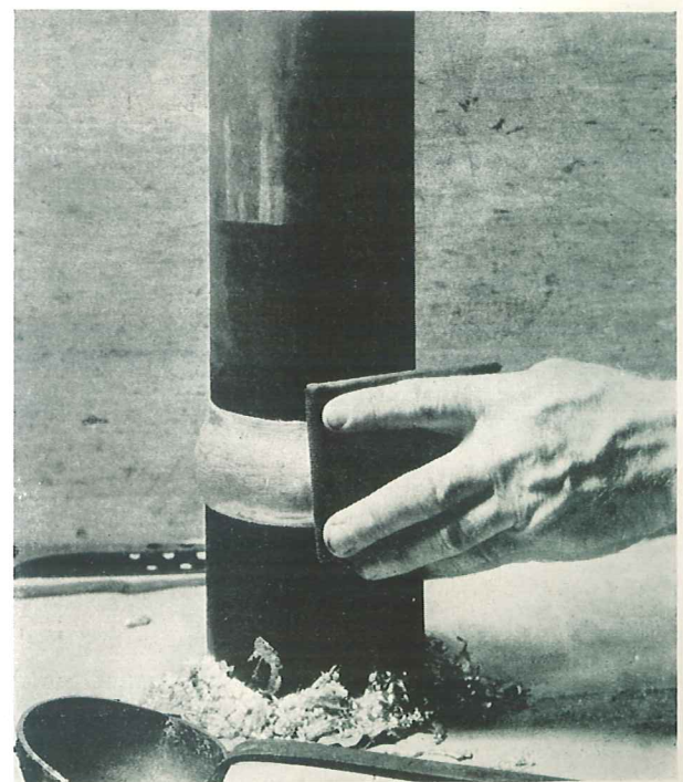
Below: Finishing a wiped joint in lead pipe.
