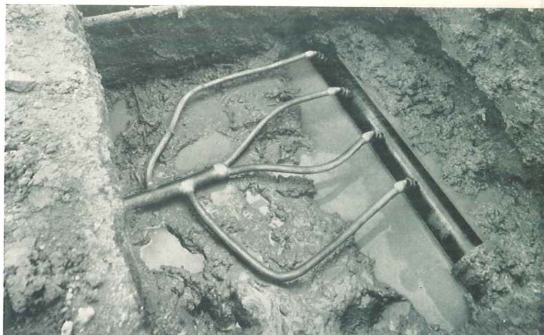
Above: Typical lead water service showing the multiple tapping method employed when a large service is connected to a small main. Below: Lead roughing-in for a battery of four lavatories.
