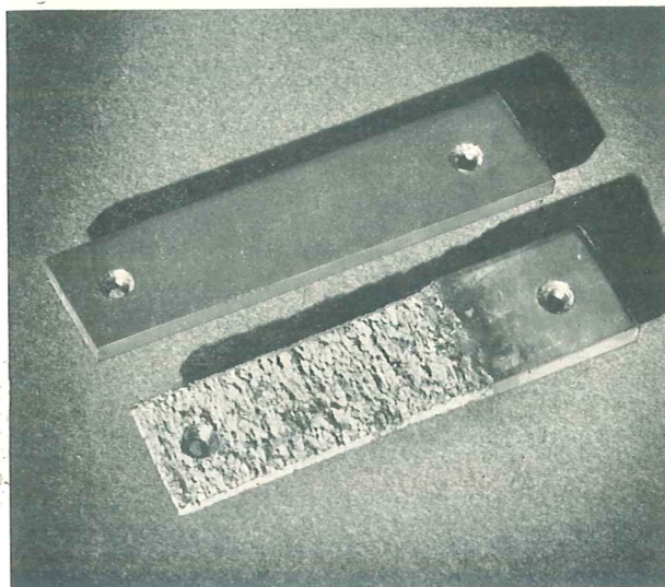
Strips of lead with and without tellurium content after immersion in 96% sulphuric acid at 305°C. for 3 minutes. Tellurium lead weight loss, 0.97%—other lead 5.11%.
