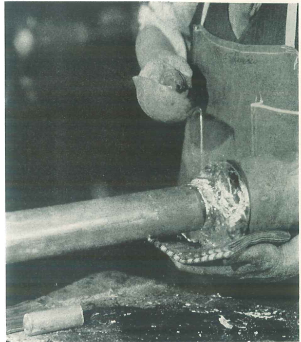
Above: Pouring molten solder over a joint in a lead-covered telephone cable. As the solder cools to a plastic state, it is molded to shape with the "catch cloth."
