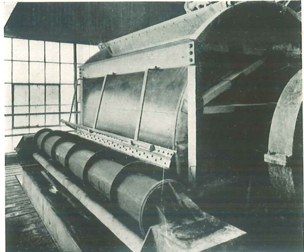
Above: Lead covered drum-type acid filter in a pigment manufacturing plant. The trough in the foreground is also formed from sheet lead. The revolving drum is made of perforated lead.
