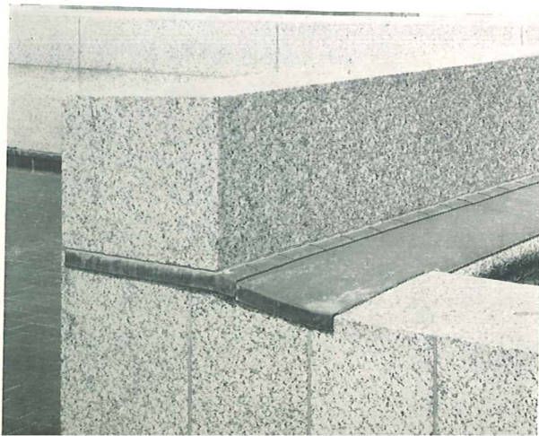
Below: This photograph shows a lead-covered cornice and through-wall flashing. The cornice covering has been attached to the flashing with a loose-locked seam.
