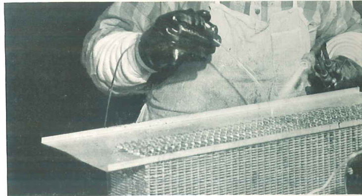
Torch soldering operation on autotruck radiator.
