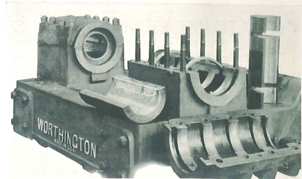
Above: Ring oiling pinion shaft bearings on a horizontal power pump (housing in foreground removed to show rings.)
