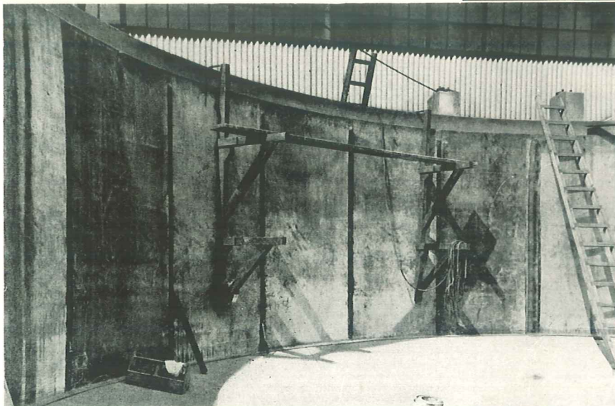
Above: Lead covered drum-type acid filter in a pigment manufacturing plant. The trough in the foreground is also formed from sheet lead. The revolving drum is made of perforated lead.
