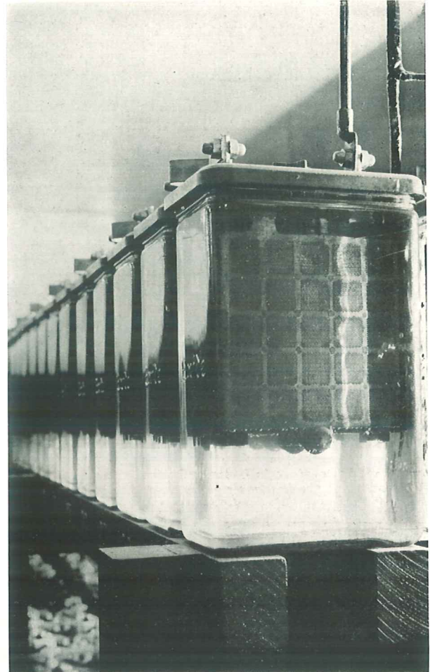
Above: Storage battery room in a large broadcasting studio. Note the lead grid inside the battery in the foreground. Below: Standard type of grid used in the automobile storage battery. The grid at the right is shown after pasting with lead oxide.
